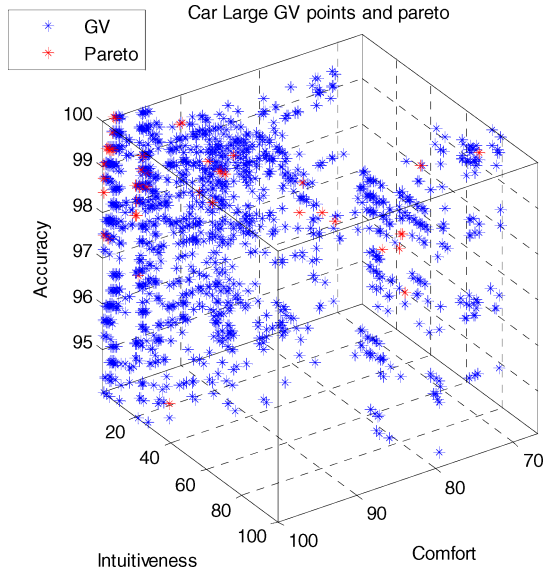
Fig. 8. 3D plot of the MOP GV and Pareto solutions obtained using a semi-complete search.
