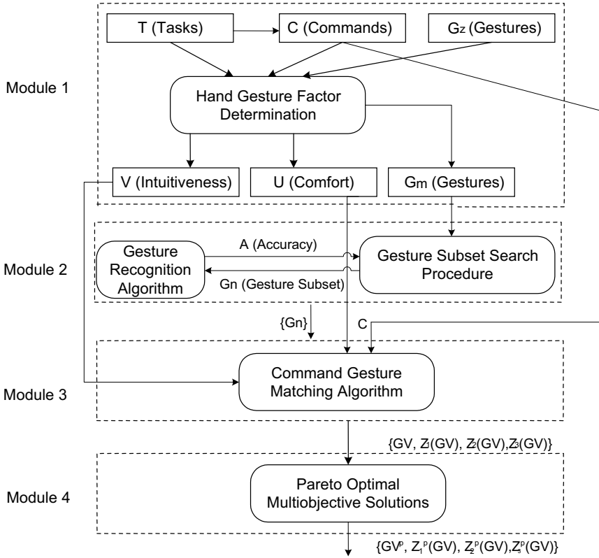
Fig. 1. Architecture of optimal hand gesture vocabulary solution procedure.
