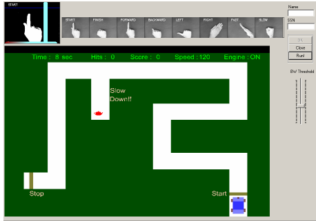
Fig. 10. Gesture car control task screen.
